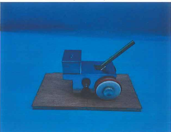
During paint film hardness test
