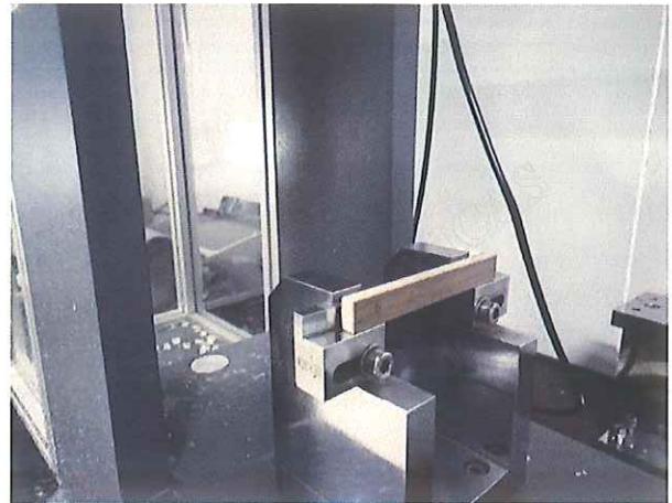
During impact strength test
