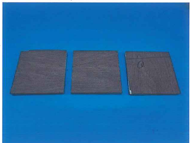
After paint film hardness test
